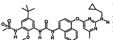
N-[5-tert-Butyl-3-(3-{4-[2-(cyclopropylmethyl-amino)-6-methyl-pyrimidin-4-yloxy]-naphthalen-1-yl]-ureido)-2-methoxy-phenyl]-methanesulfonamide;
